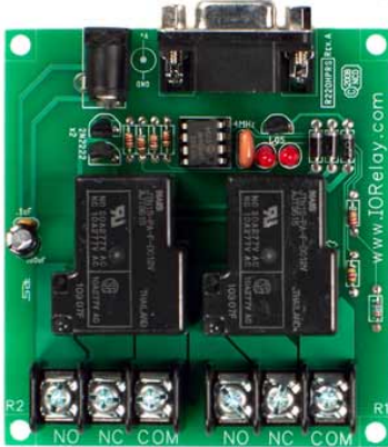
R220HPRS Serial Controller Board
